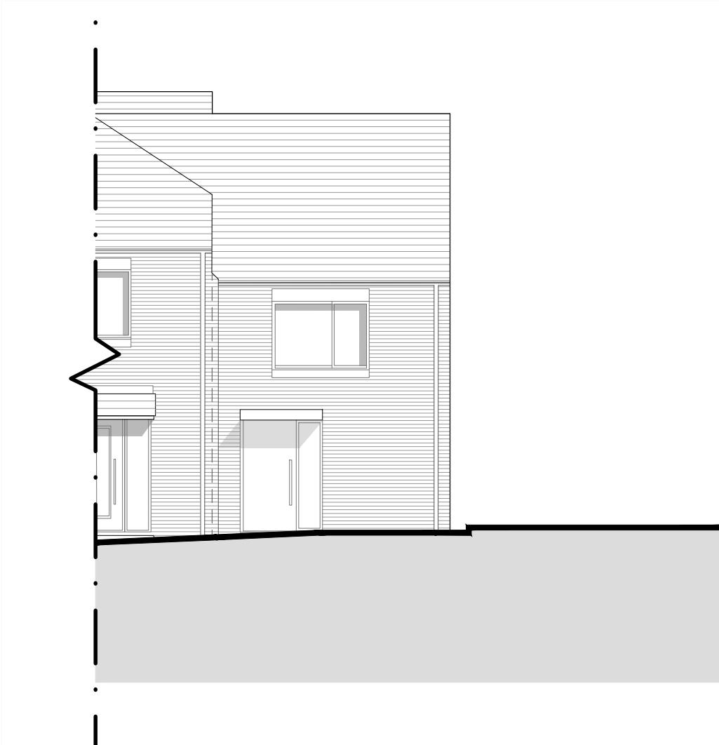
Front Elevation @1:100
