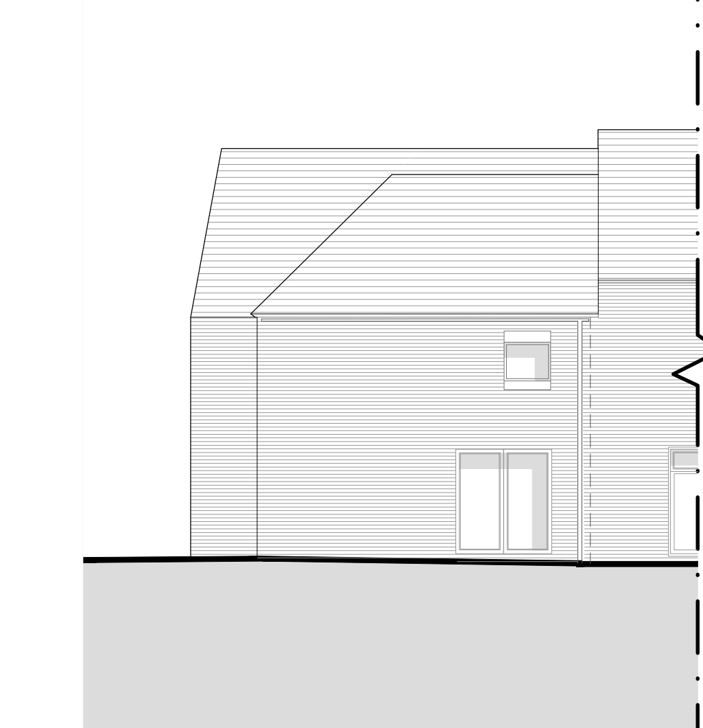
Rear Elevation @1:100
