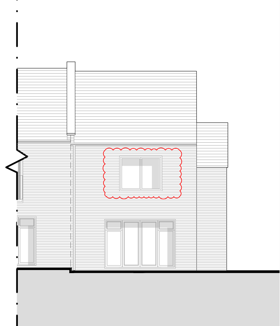
Rear Elevation @1:100
