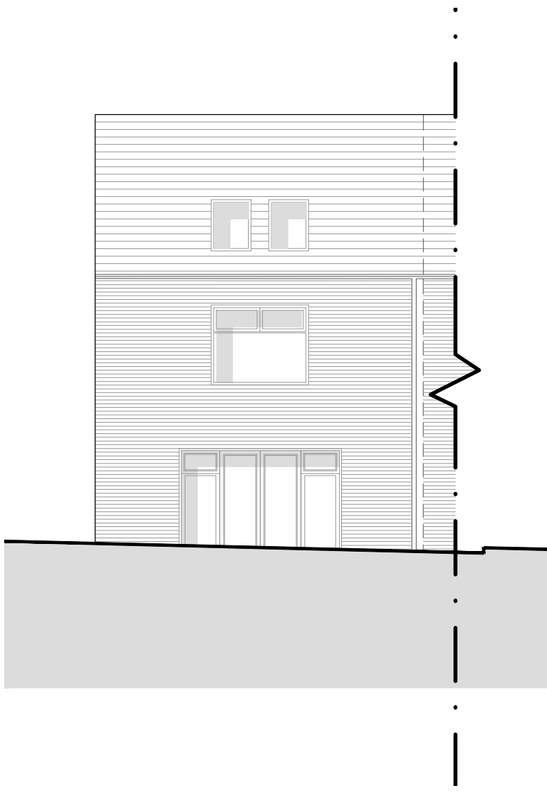
Rear Elevation @1:100
