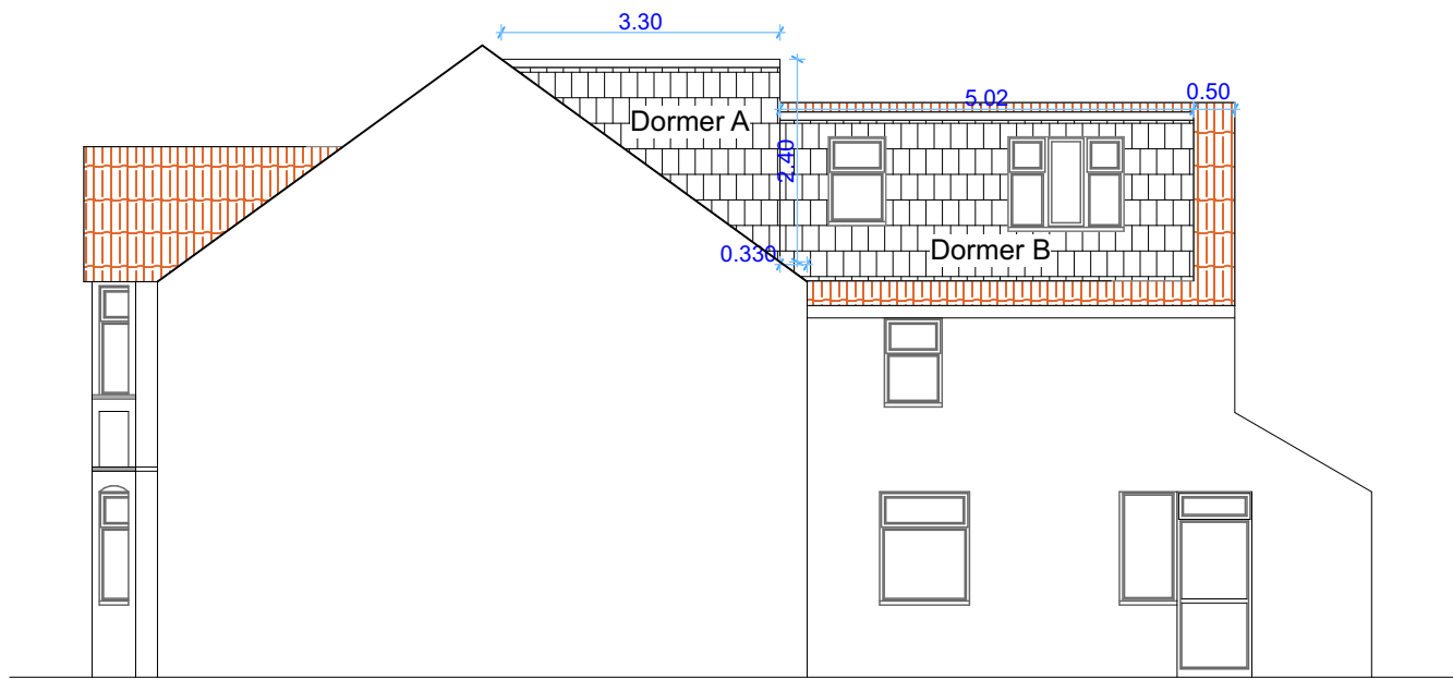
PROPOSED SIDE ELEVATION - A
