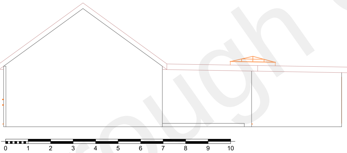
8 West Elevation Proposed 1:100
