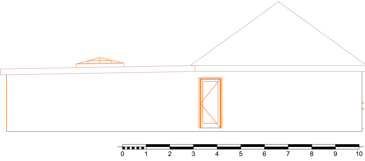
7 East Elevation Proposed 1:100
