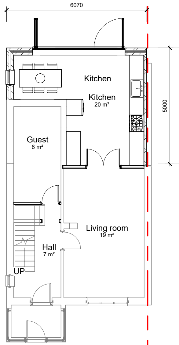
GF - Proposed 1 : 100
