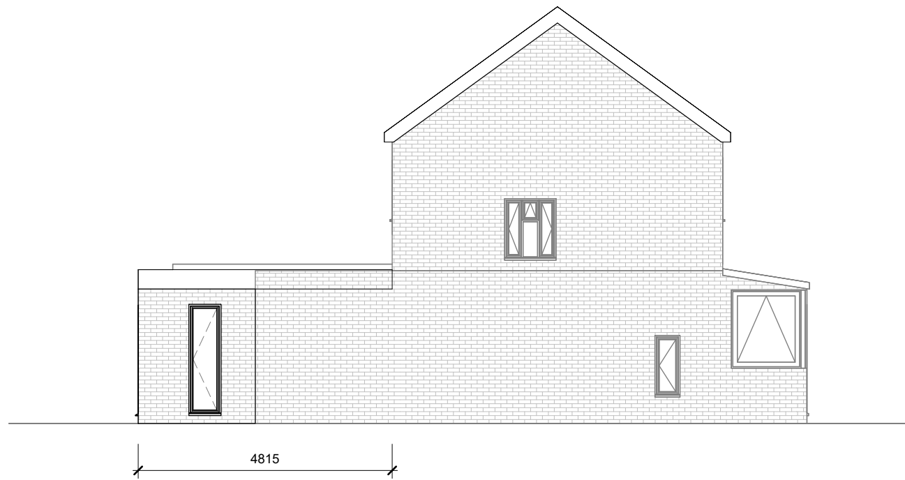
West - Proposed 1 : 100
