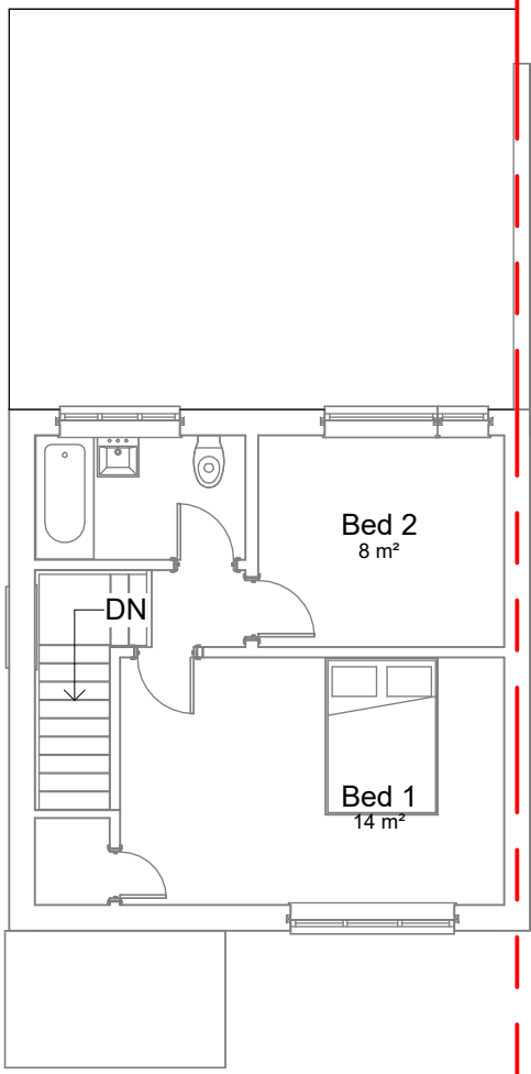
FF - Proposed 1 : 100
