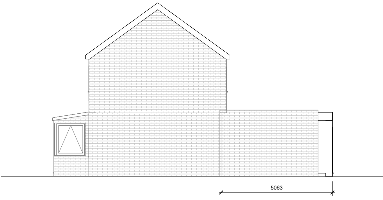
East - Proposed 1 : 100
