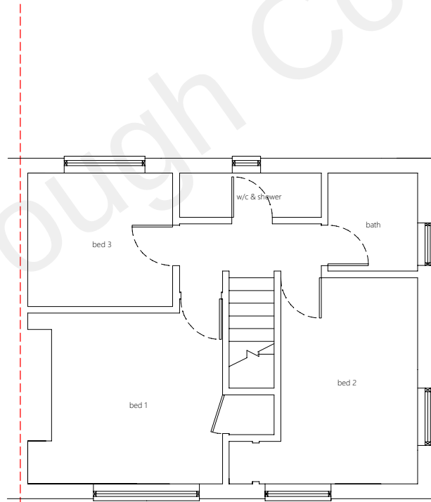
1st Floor Existing Layout 1:100
