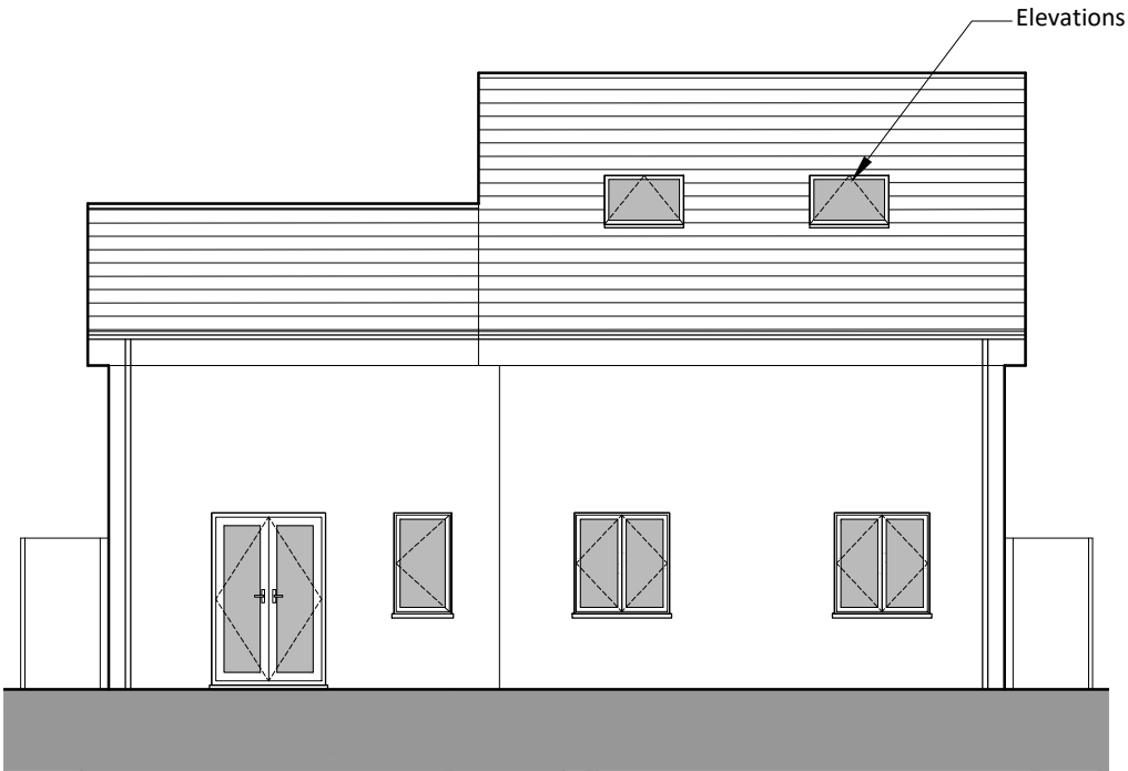
Proposed Rear (South) Elevation 1:100
