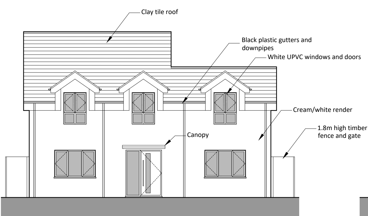
Proposed Front (North) Elevation 1:100
