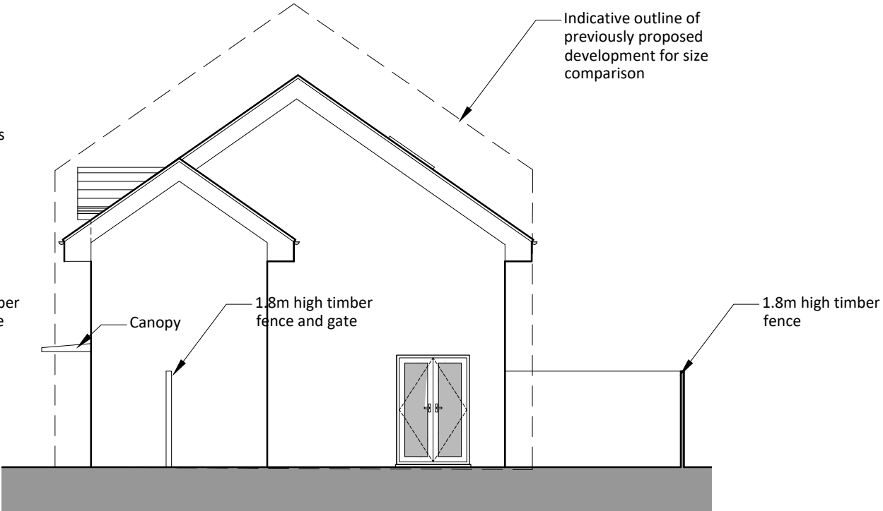
Proposed Side (West) Elevation 1:100
