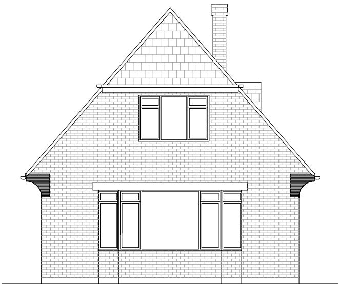
Existing north
