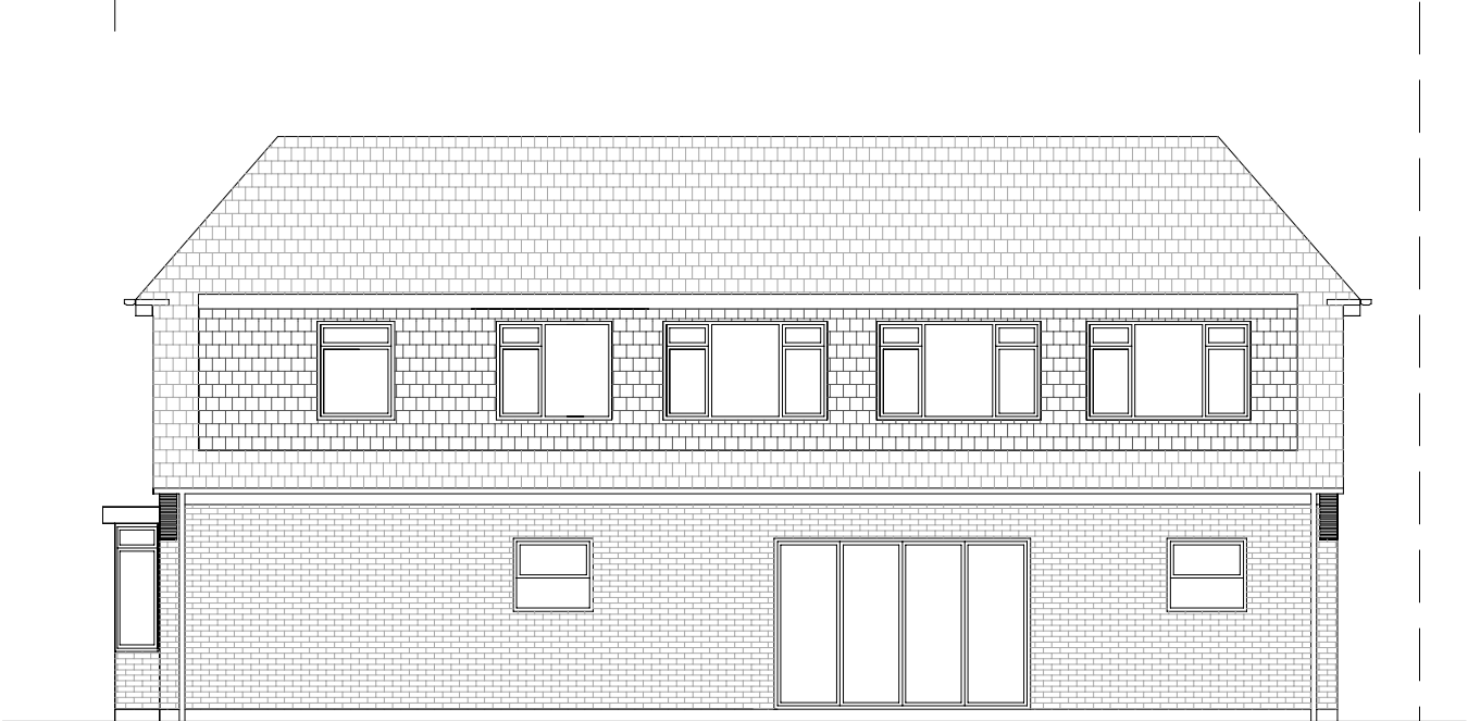
Proposed west
