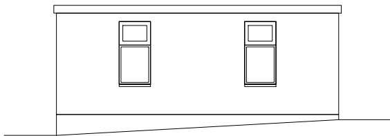
Existing Right Hand Side Elevation
