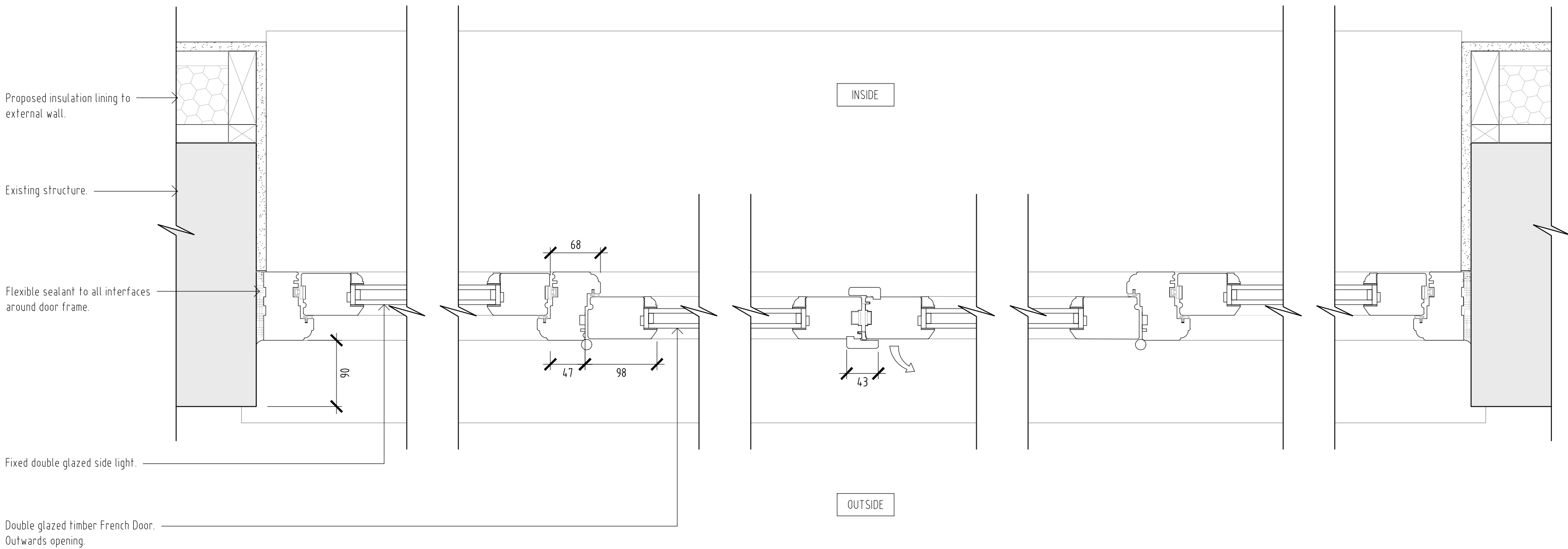
Double glazed timber french doors with sidelights jamb detail
