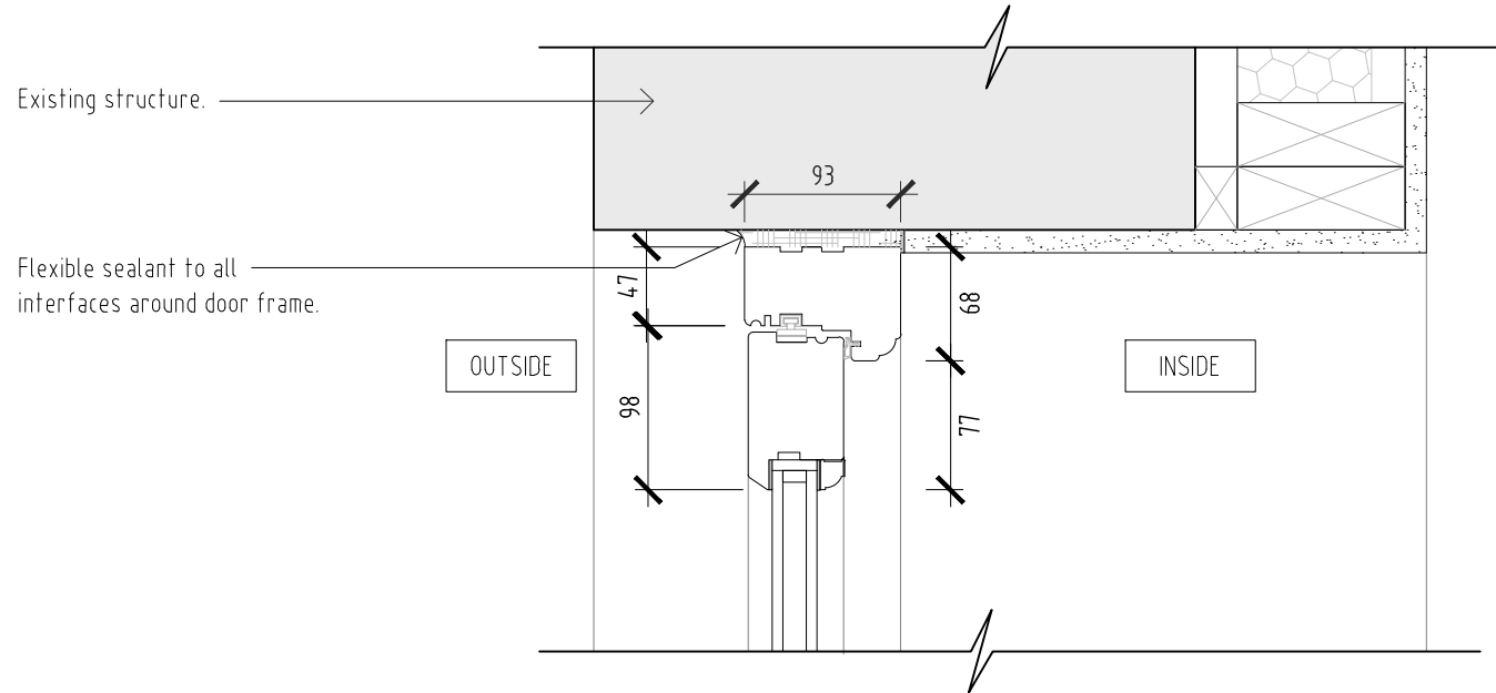
Double glazed timber french doors head detail
