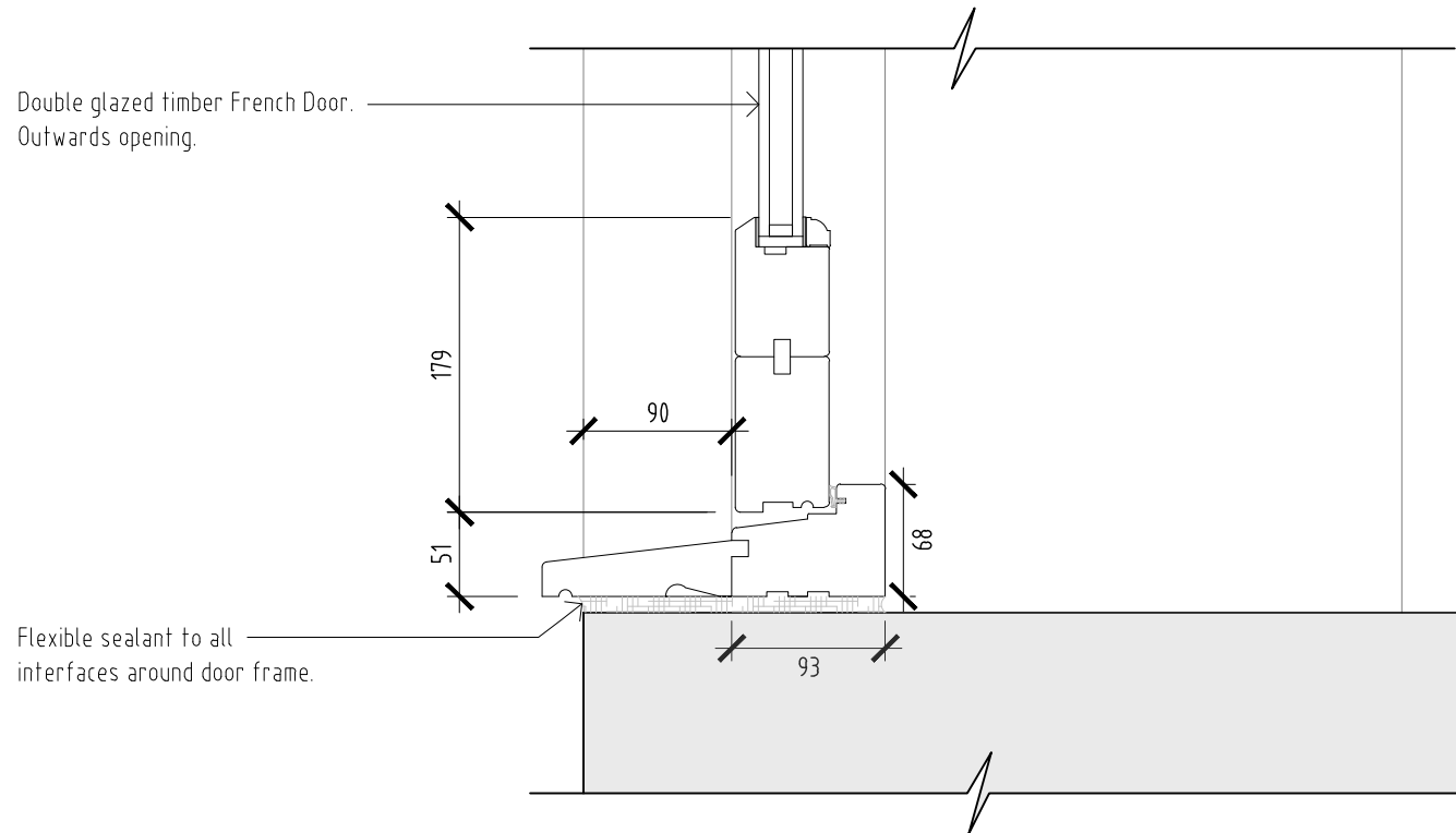
Double glazed timber french doors cill detail
