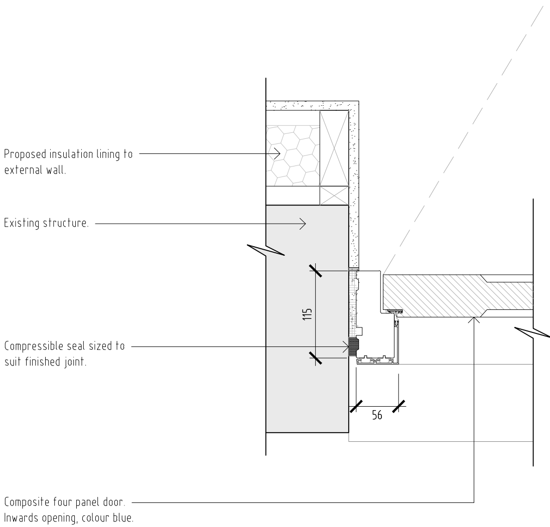
Composite front door jamb detail
