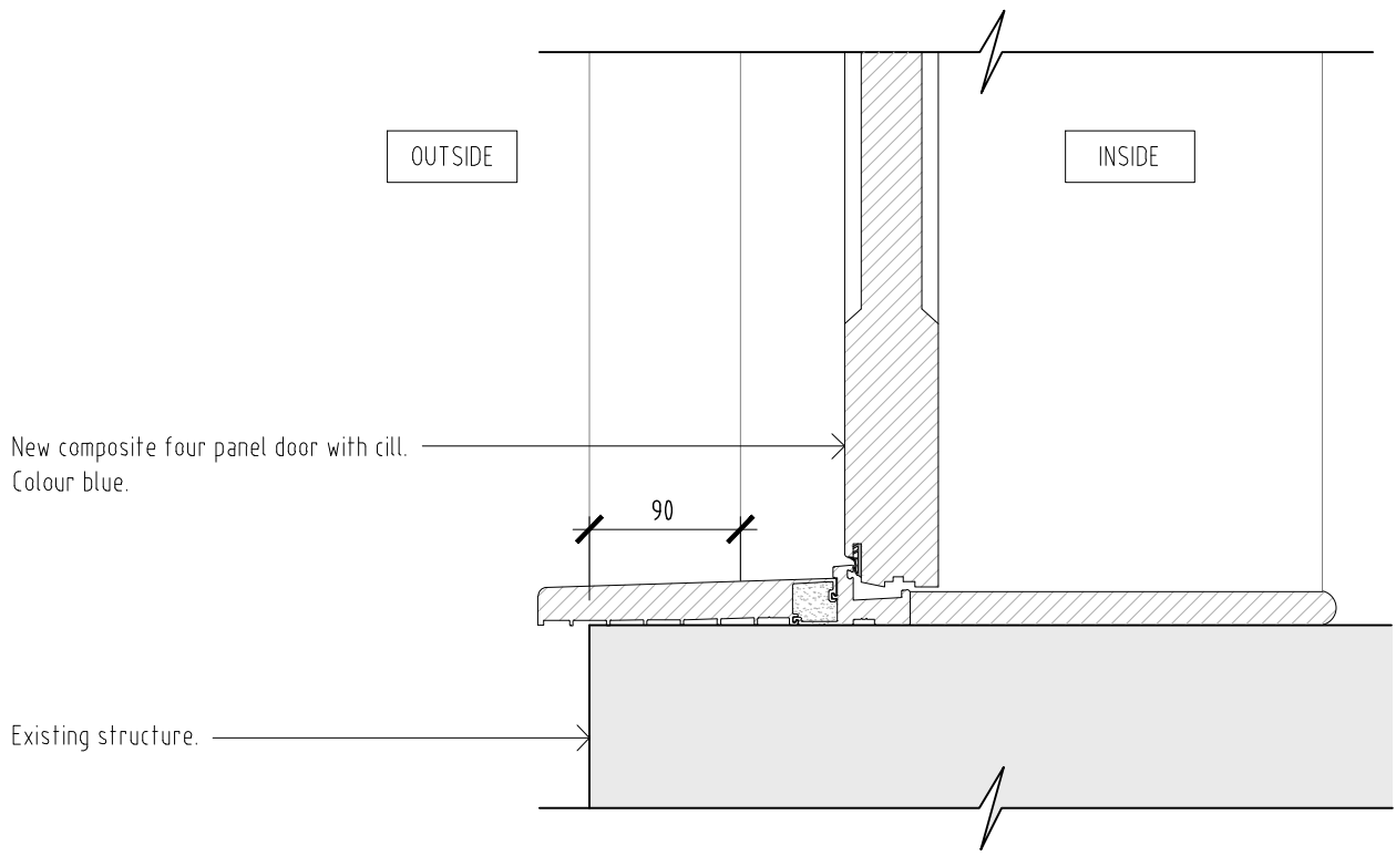
Composite front door cill detail
