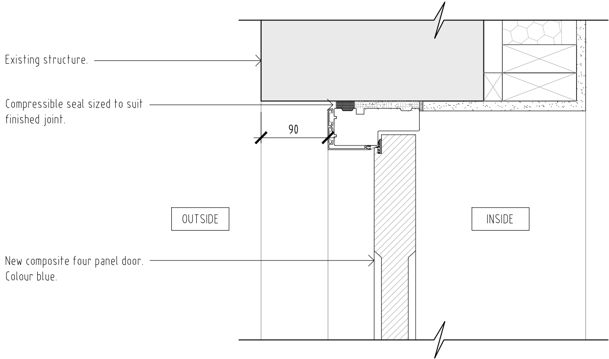
Composite front door head detail
