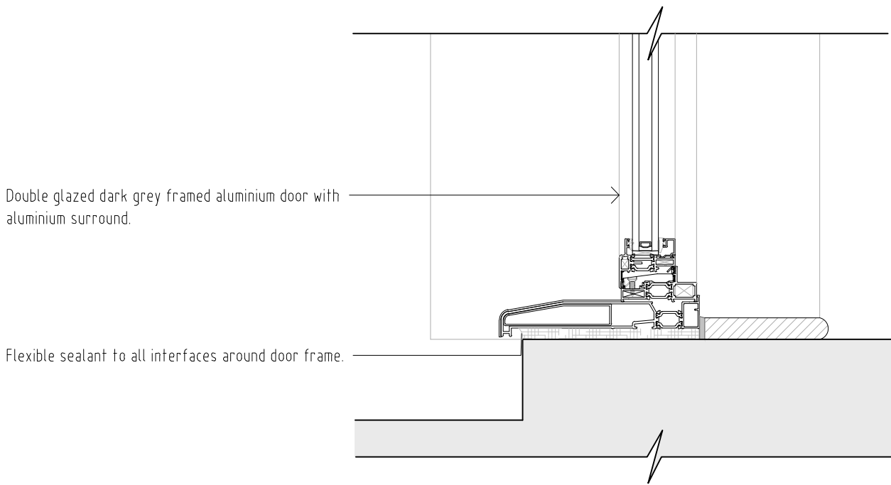
Double glazed aluminium door with aluminium surround cill detail
