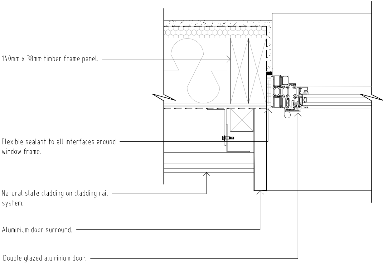
Double glazed aluminium door with aluminium surround jamb detail
