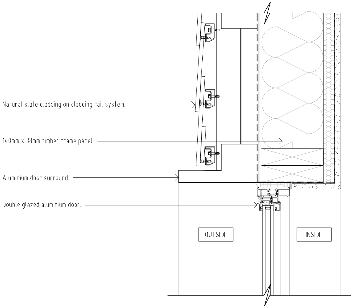
Double glazed aluminium door with aluminium surround head detail
