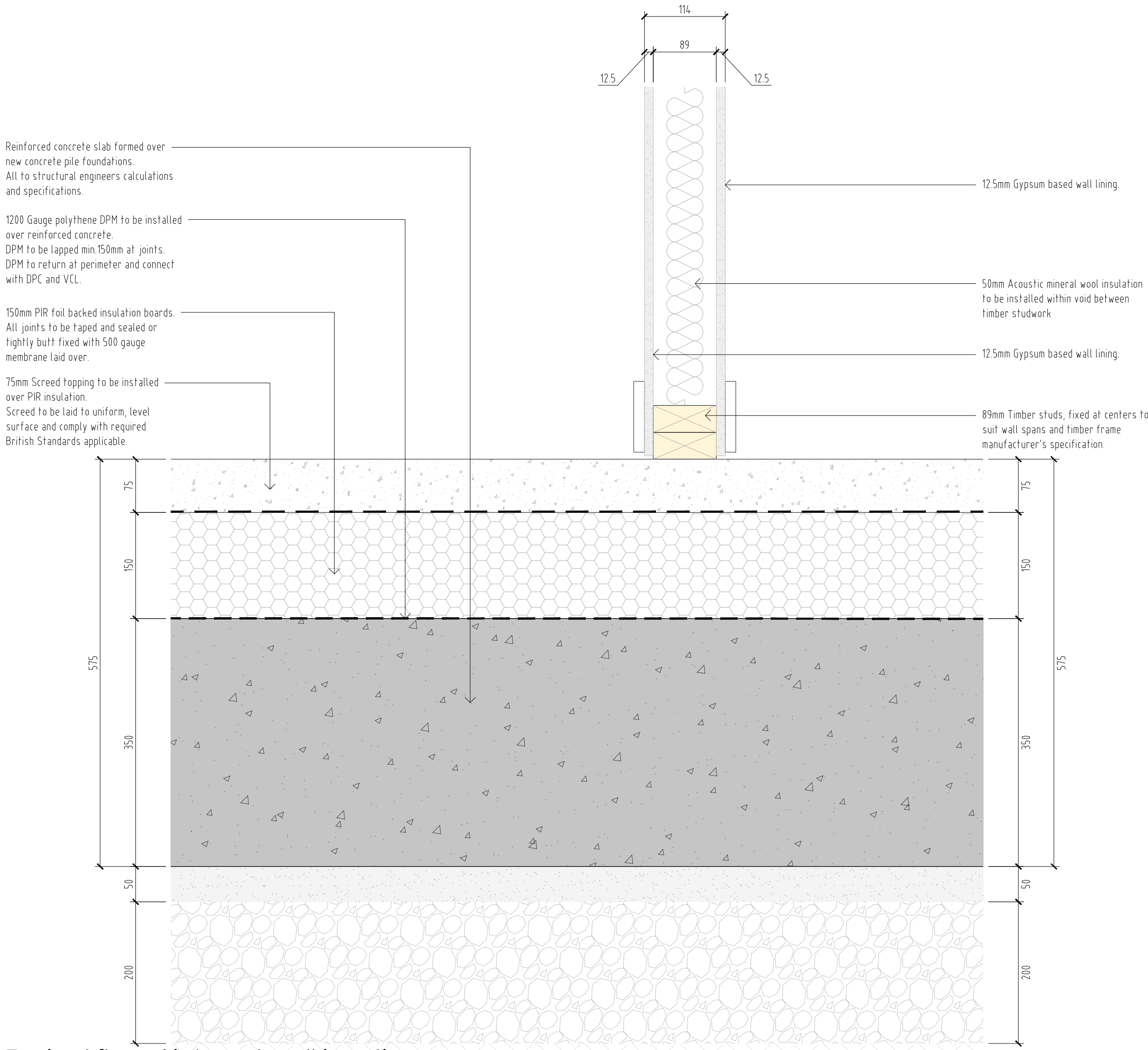
Typical floor / internal wall junction
