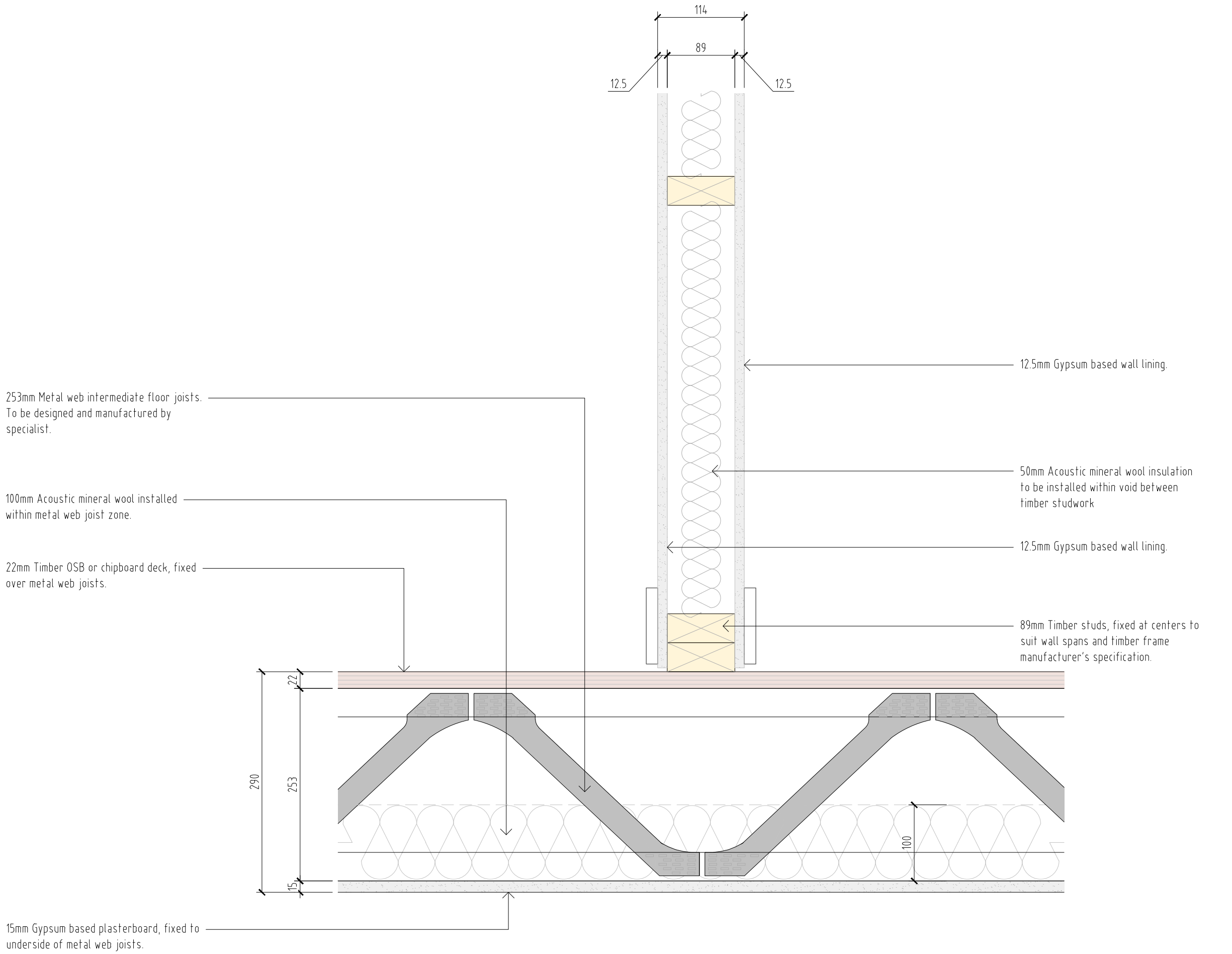
Intermediate floor / internal wall junction
