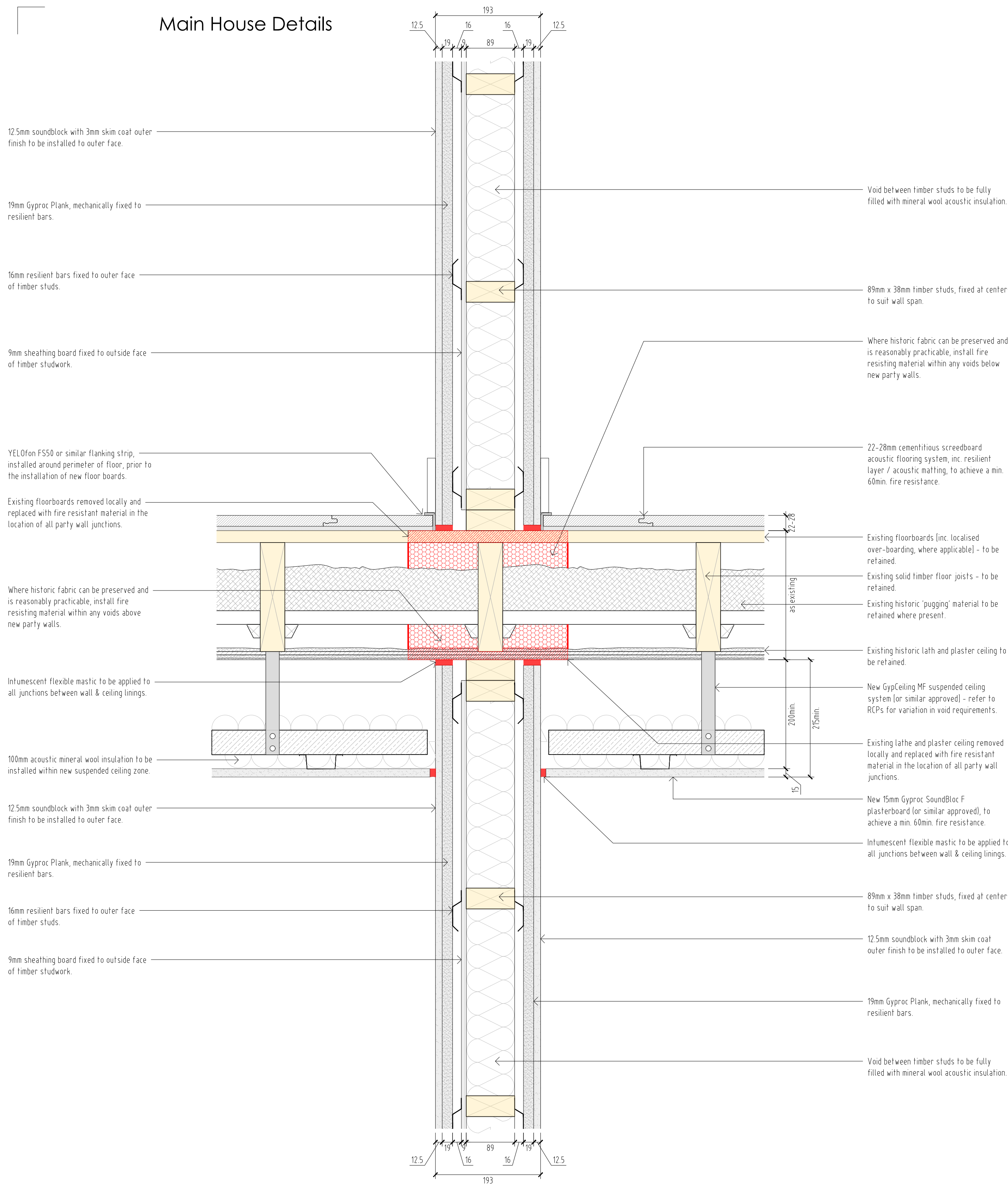
Timber separating floor / party wall junction
