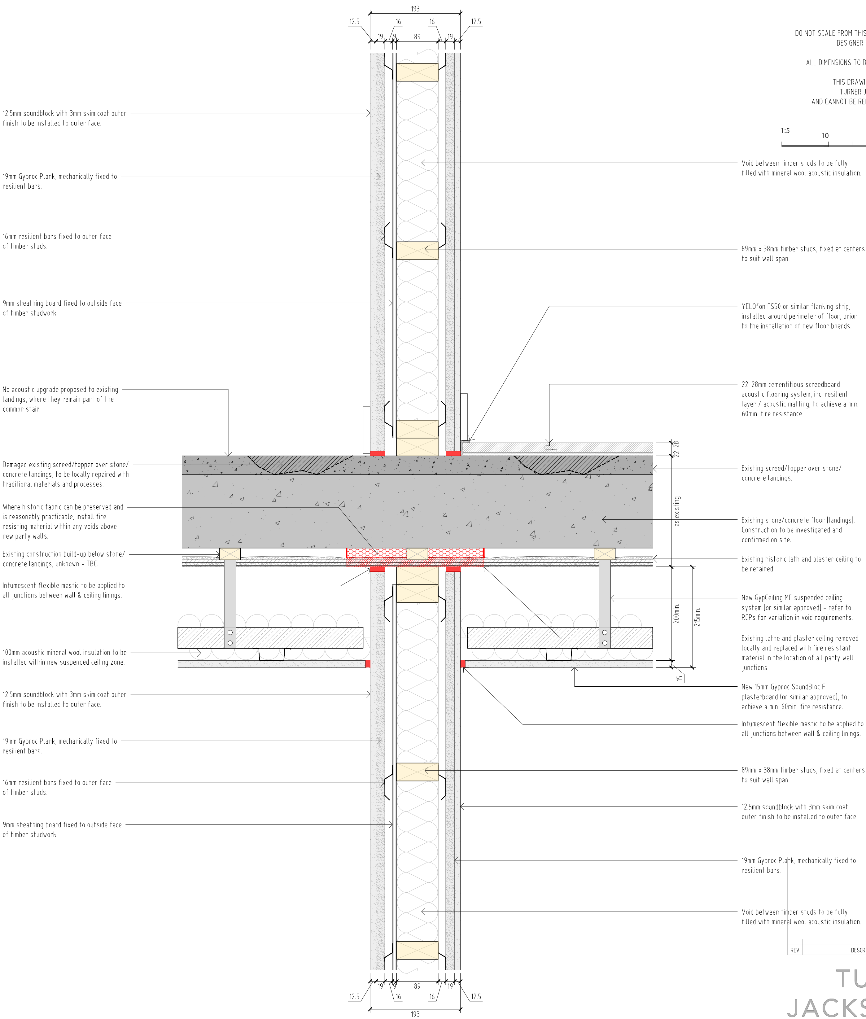
Stone / concrete separating floor / party wall junction
