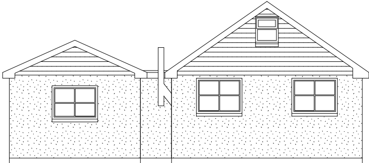
SIDE (EAST) ELEVATION
