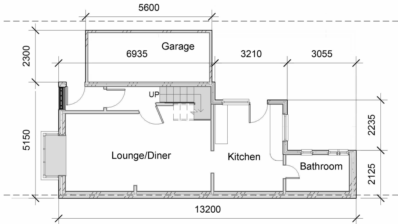
0 Ground Floor 1 : 100
