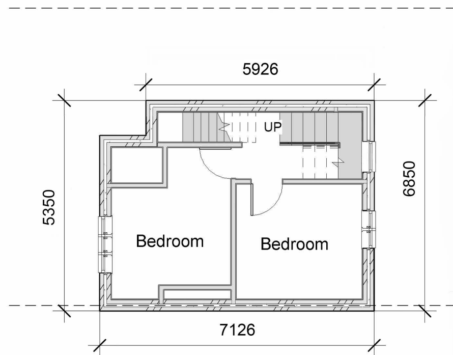
1 First Floor 1 : 100
