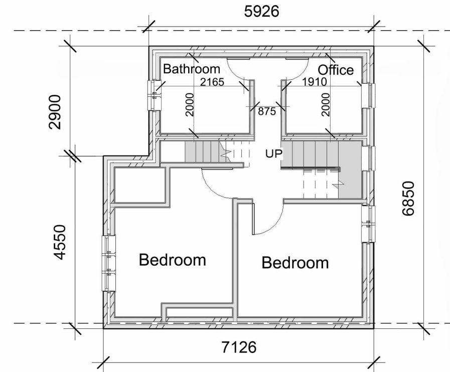
1 First Floor 1 : 100
