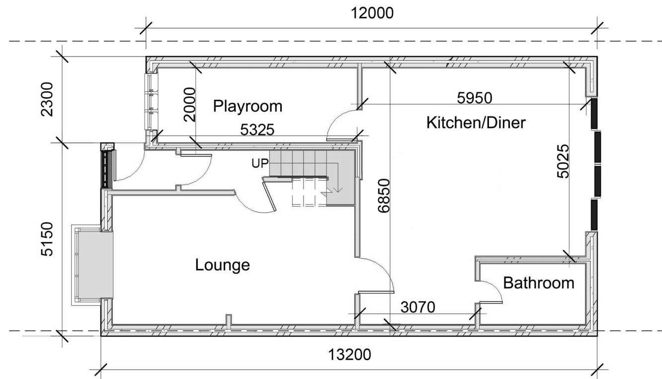
0 Ground Floor 1 : 100
