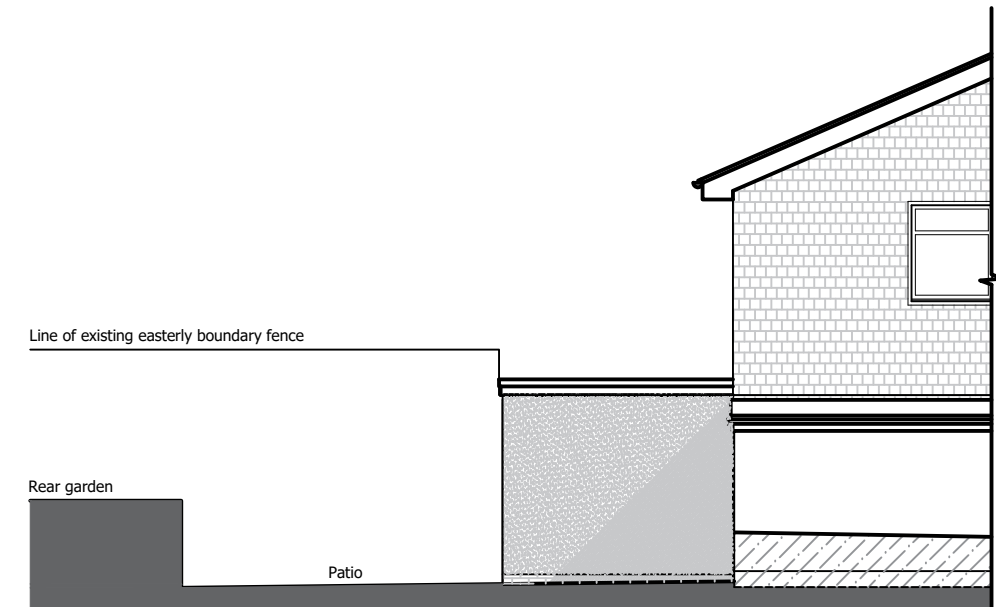
SIDE ELEVATION (Easterly facing)
