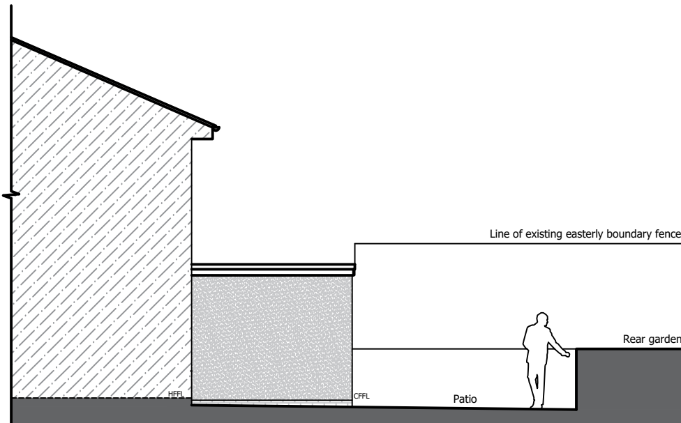
SIDE ELEVATION (Westerly facing)
