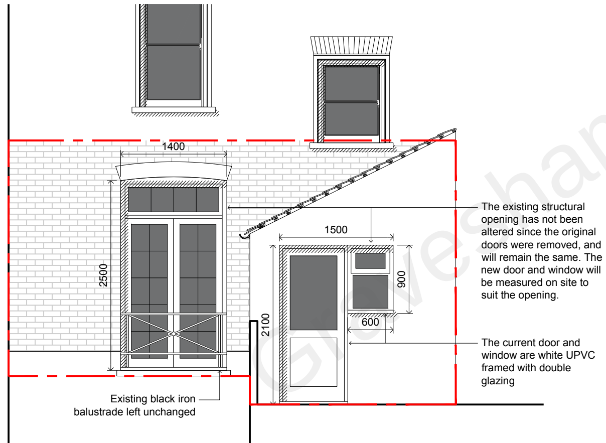
03 | 1:50 | EXISTING REAR ELEVATION
