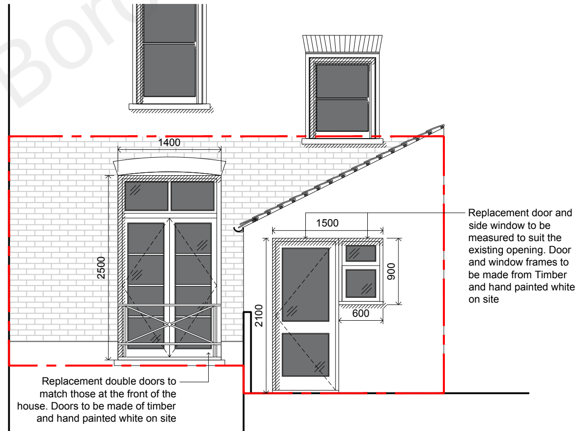
04 | 1:50 | PROPOSED REAR ELEVATION SCALE 1:50 10m
