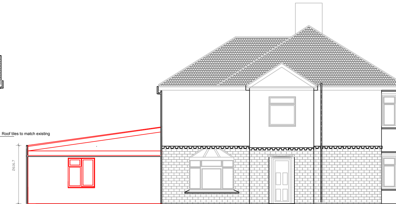
Proposed Northern Elevation
