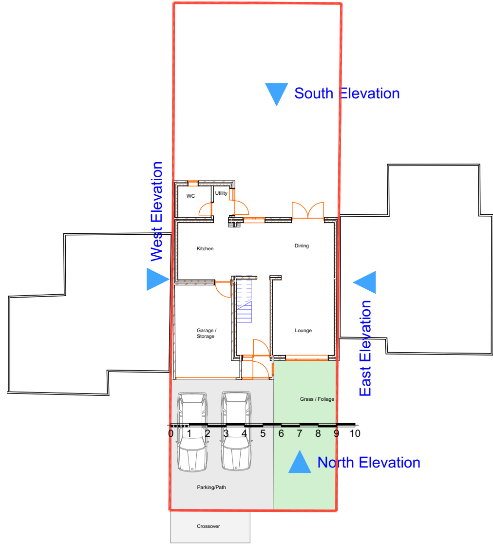
2 Site Plan Existing 1:200
