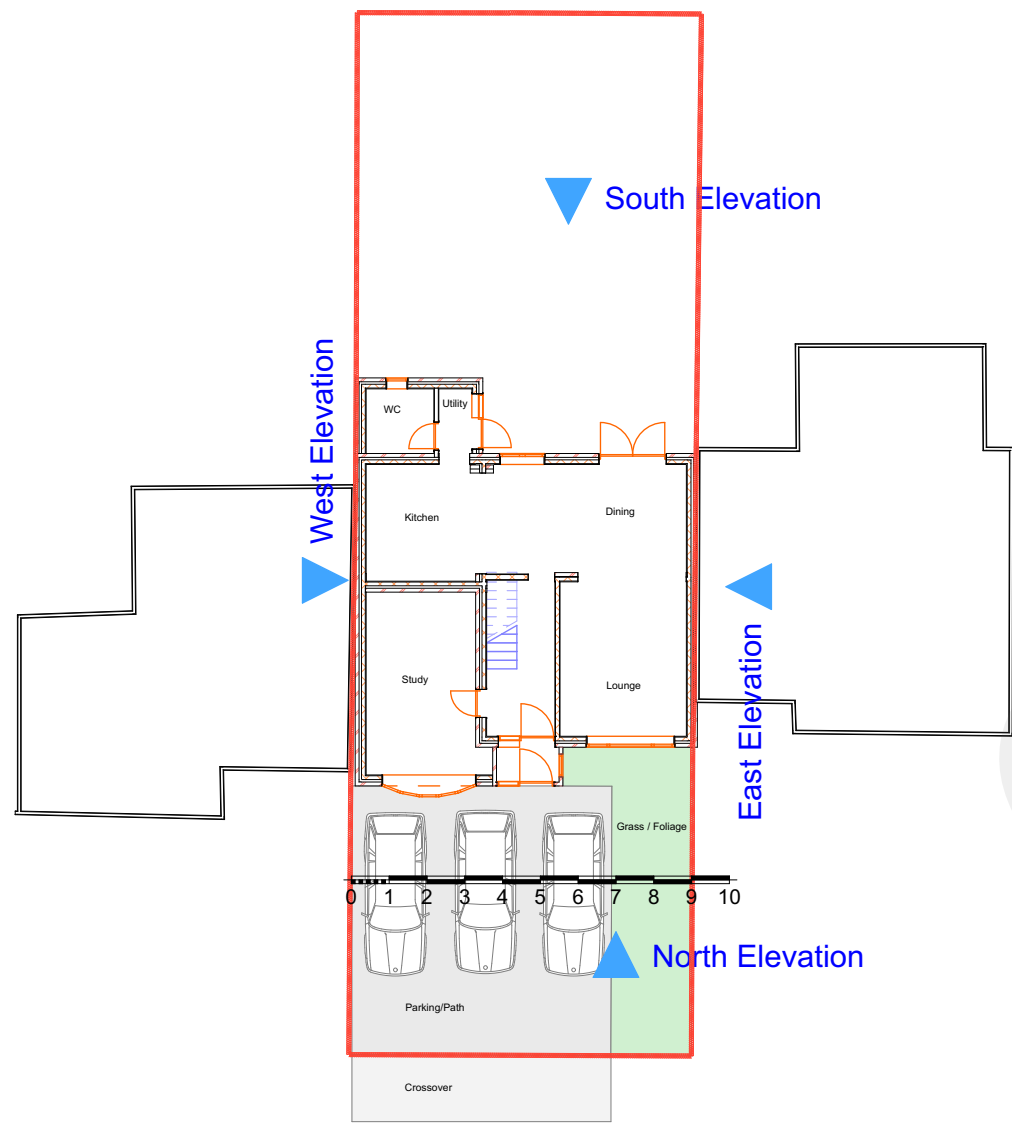
3 Site Plan Proposed 1:200
