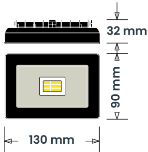
Floodlight Detail Scale 1:5
