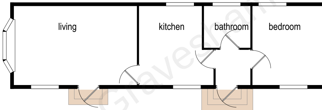
floor plan - 45 sqm internal
