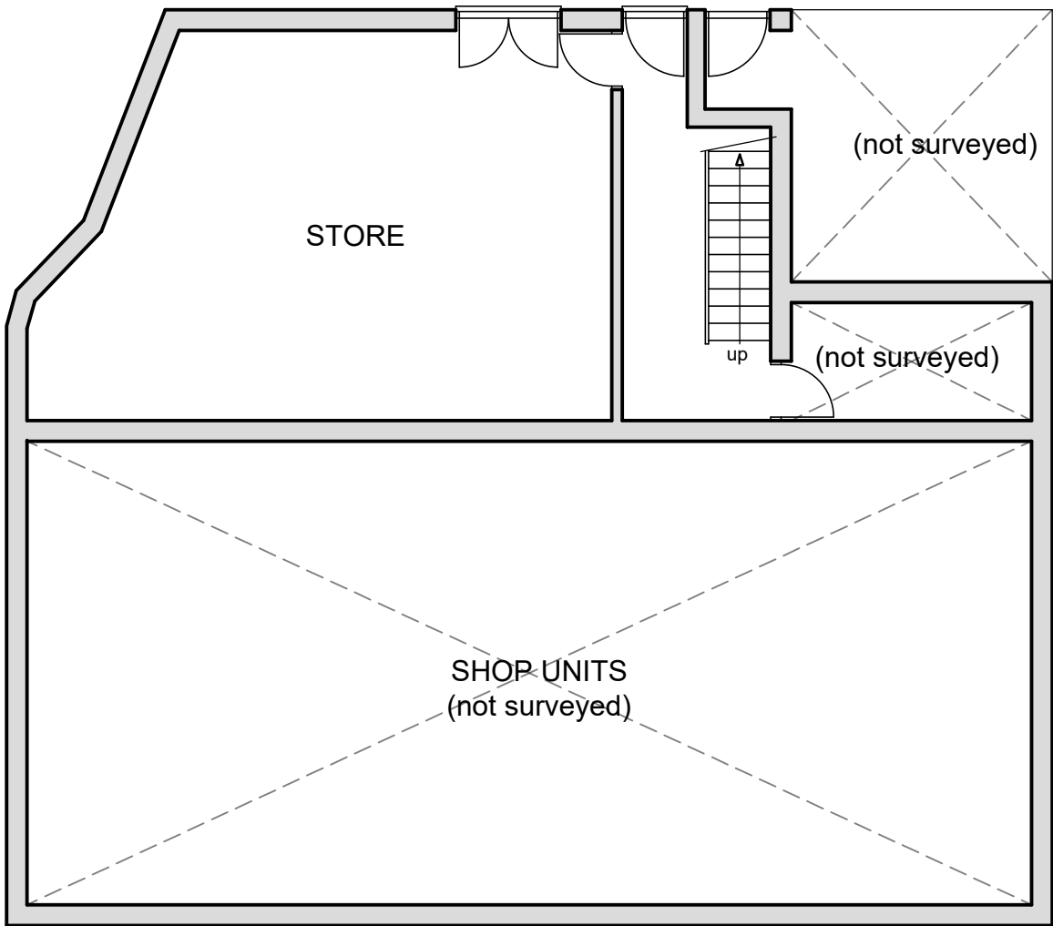
GROUND FLOOR PLAN AS PRE-EXISTING (1:100)
