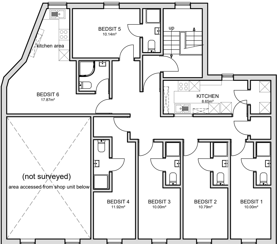
FIRST FLOOR PLAN AS PROPOSED (1:100)
