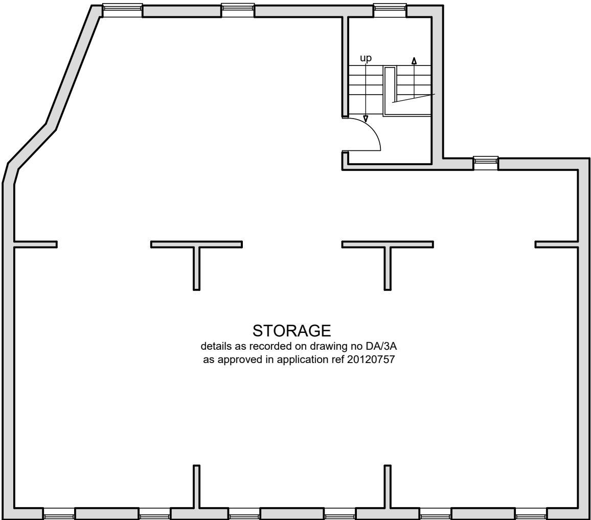
FIRST FLOOR PLAN AS PRE-EXISTING (1:100)
