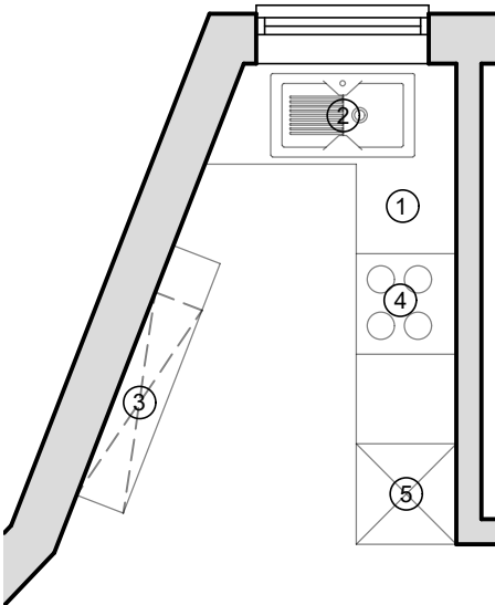
KITCHEN PLAN - BEDSIT 6 (1:50)
