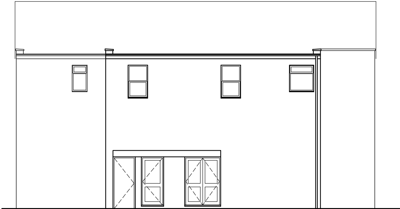
REAR ELEVATION AS PRE-EXISTING & AS PROPOSED (1:100)
