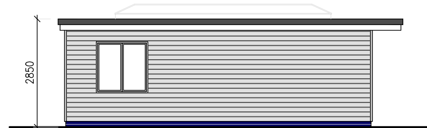
Side Elevation to 13
