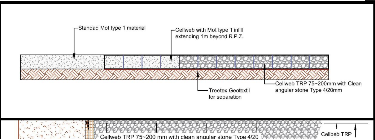
Figure 8 Cellular Confinement System - Kerb Edging
