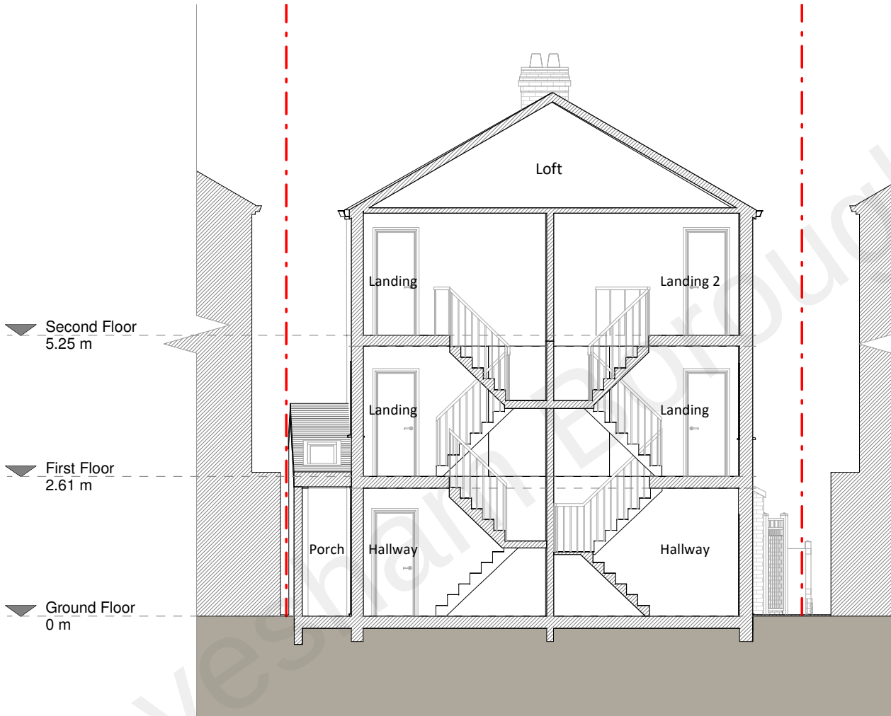
Section C - C
