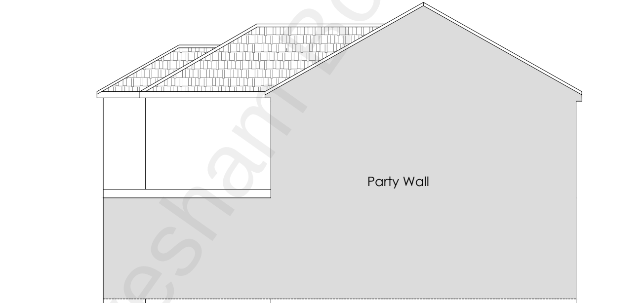
Pre-Conversion Side Elevation1
