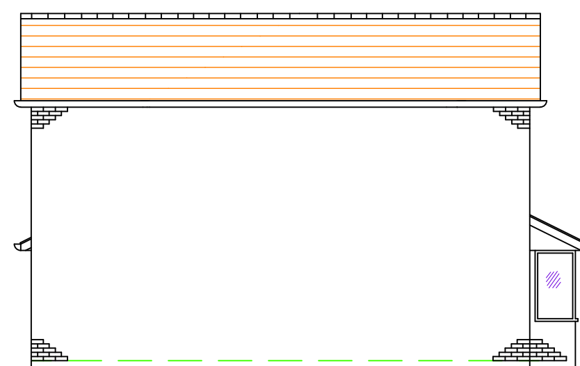
Existing Side (East) Elevation 1:100
