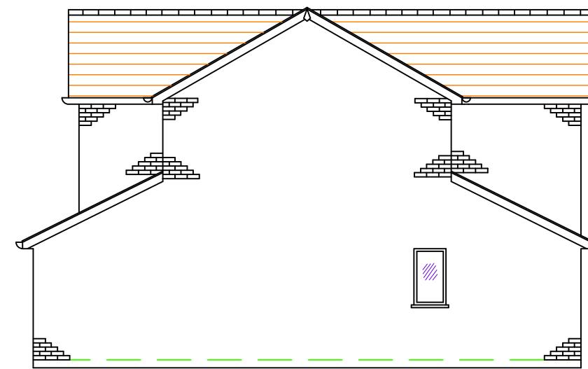
Existing Side (West) Elevation 1:100
