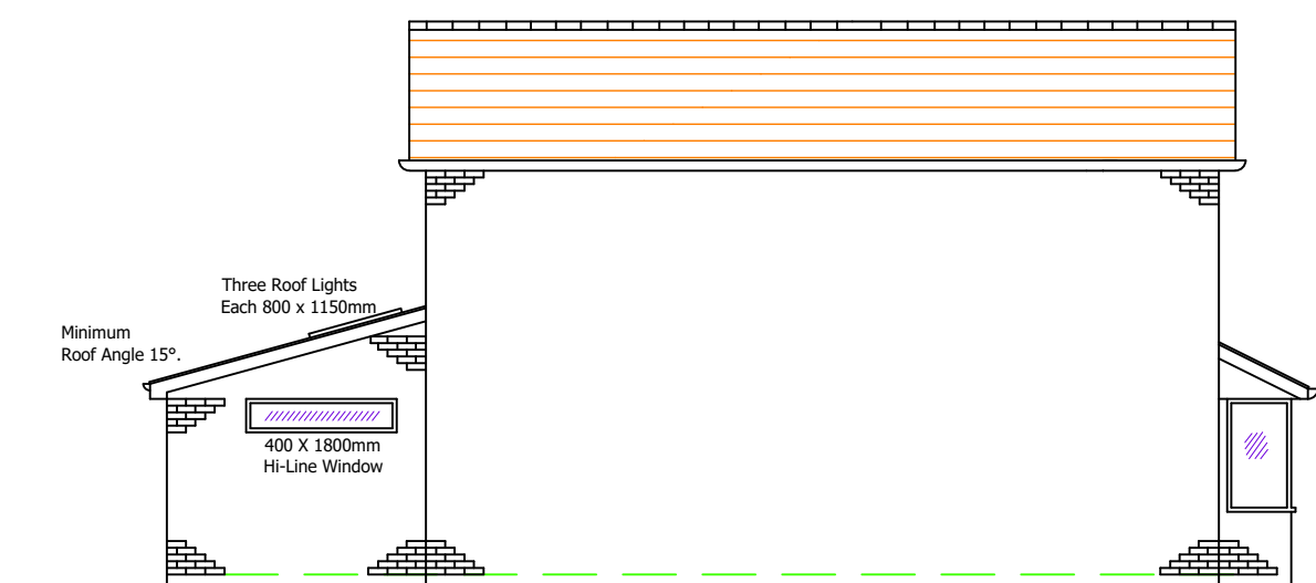
Proposed Side (East) Elevation 1:100
