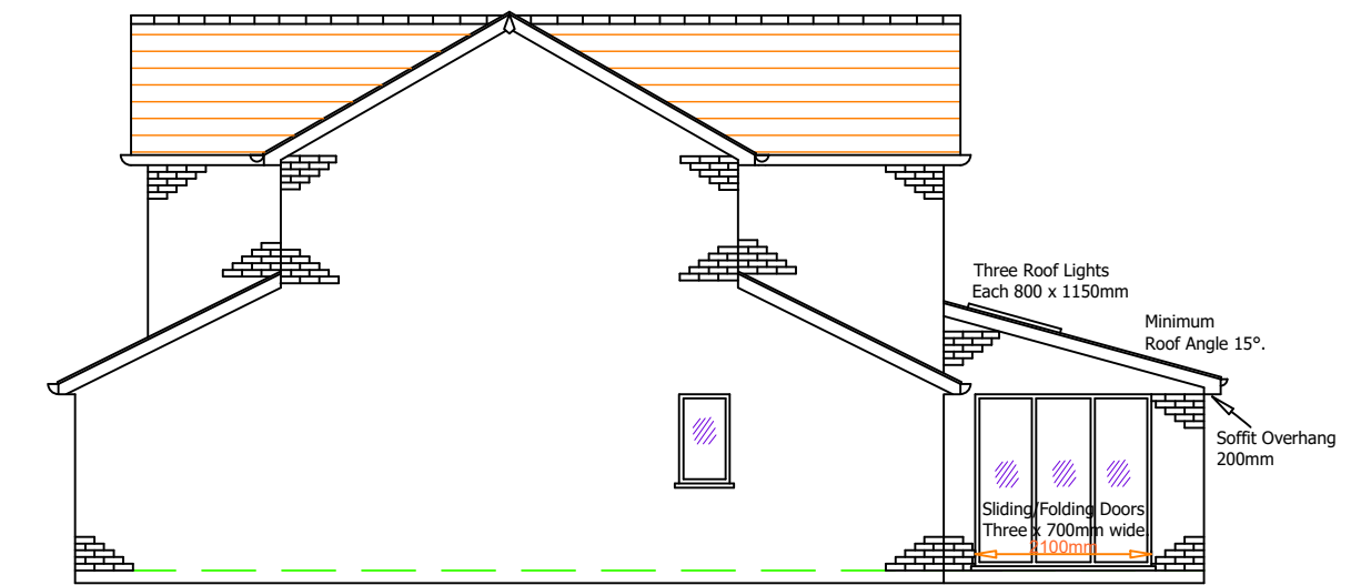
Proposed Side (West) Elevation 1:100
