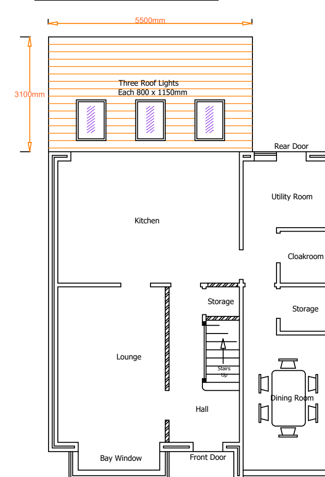
Proposed Extension Roof Plan Showing Roof Lights
