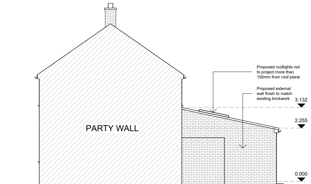
2 Side Elevation (South) 1 : 100
