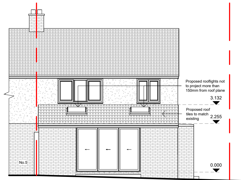
3 Rear Elevation (East) 1 : 100
