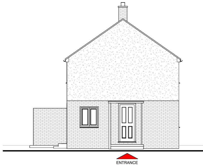
4 Side Elevation (North) 1 : 100
