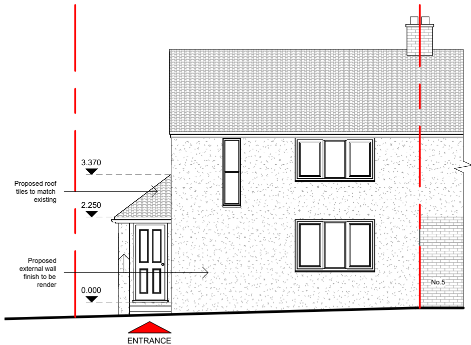
1 Front Elevation (West) 1 : 100
