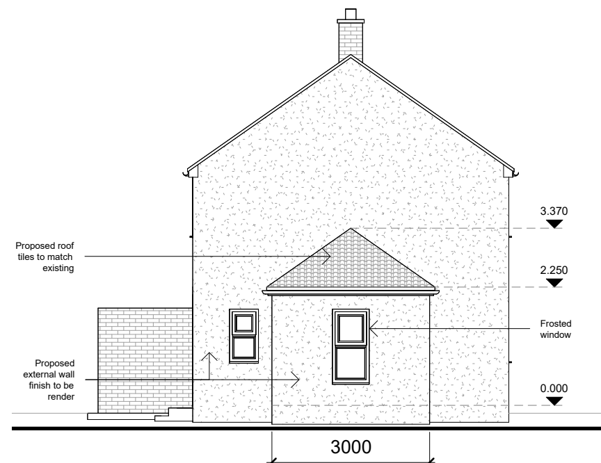
4 Side Elevation (North) 1 : 100
