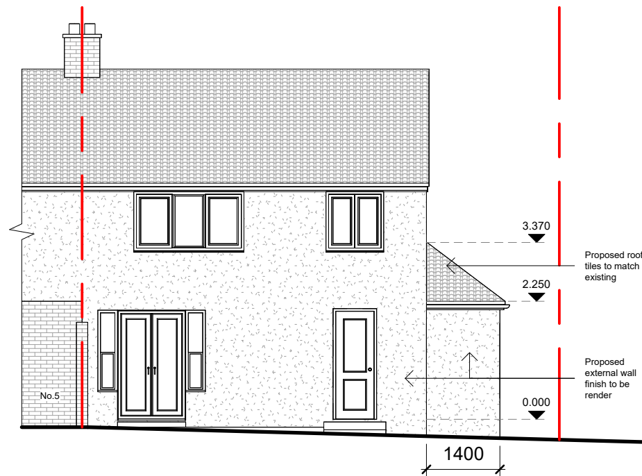
3 Rear Elevation (East) 1 : 100
