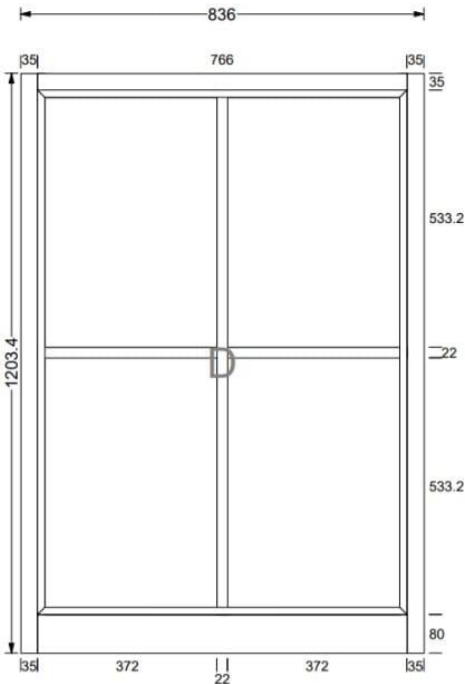
S1 Screen Casement Fixed
