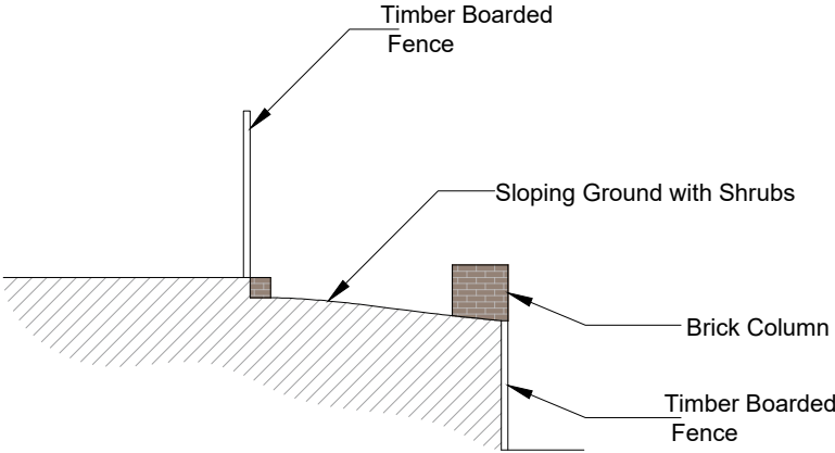
Existing Section AA' 1:100
