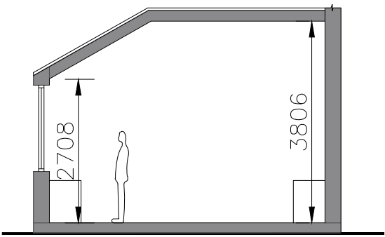
Section AA (As approved)
