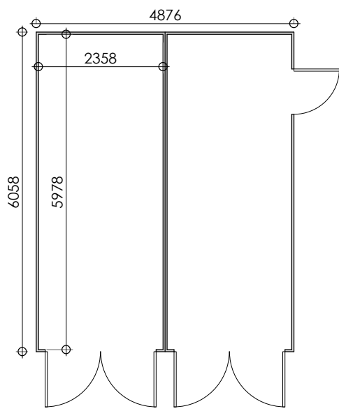
CONTAINERS - FLOOR PLAN
