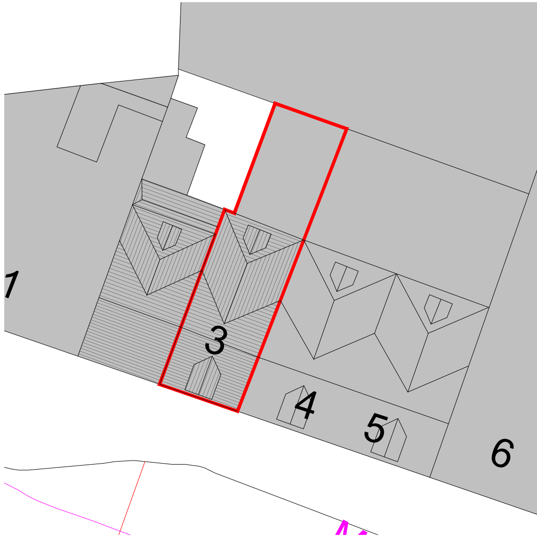
Proposed Block Plan 1:200
