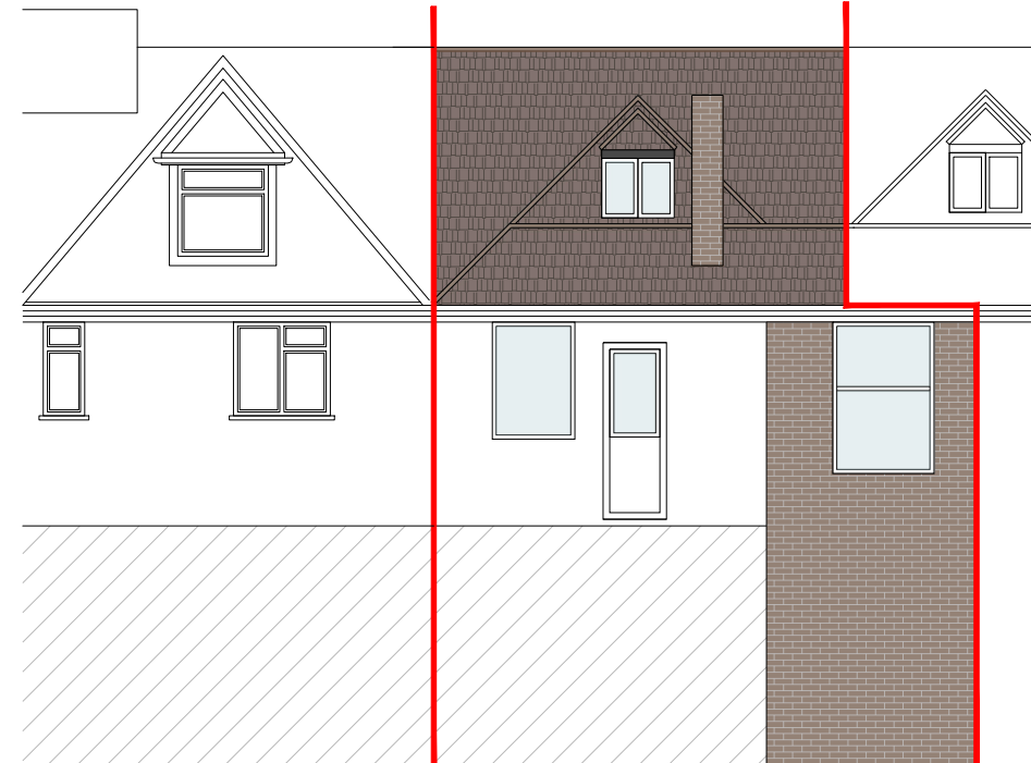
Existing North Elevation (Rear)
