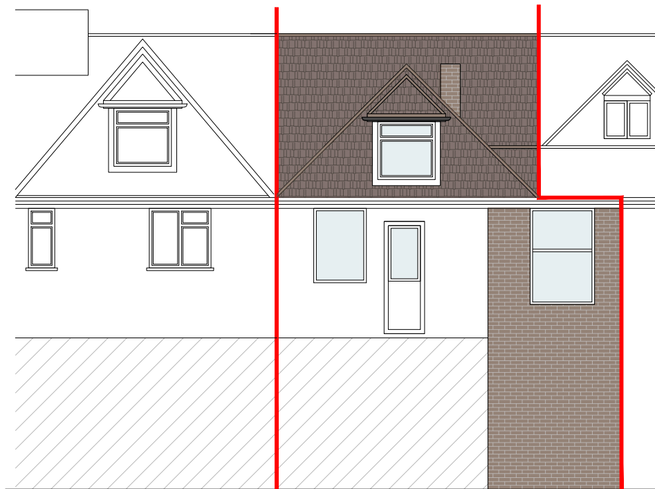
Proposed North Elevation (Rear)
