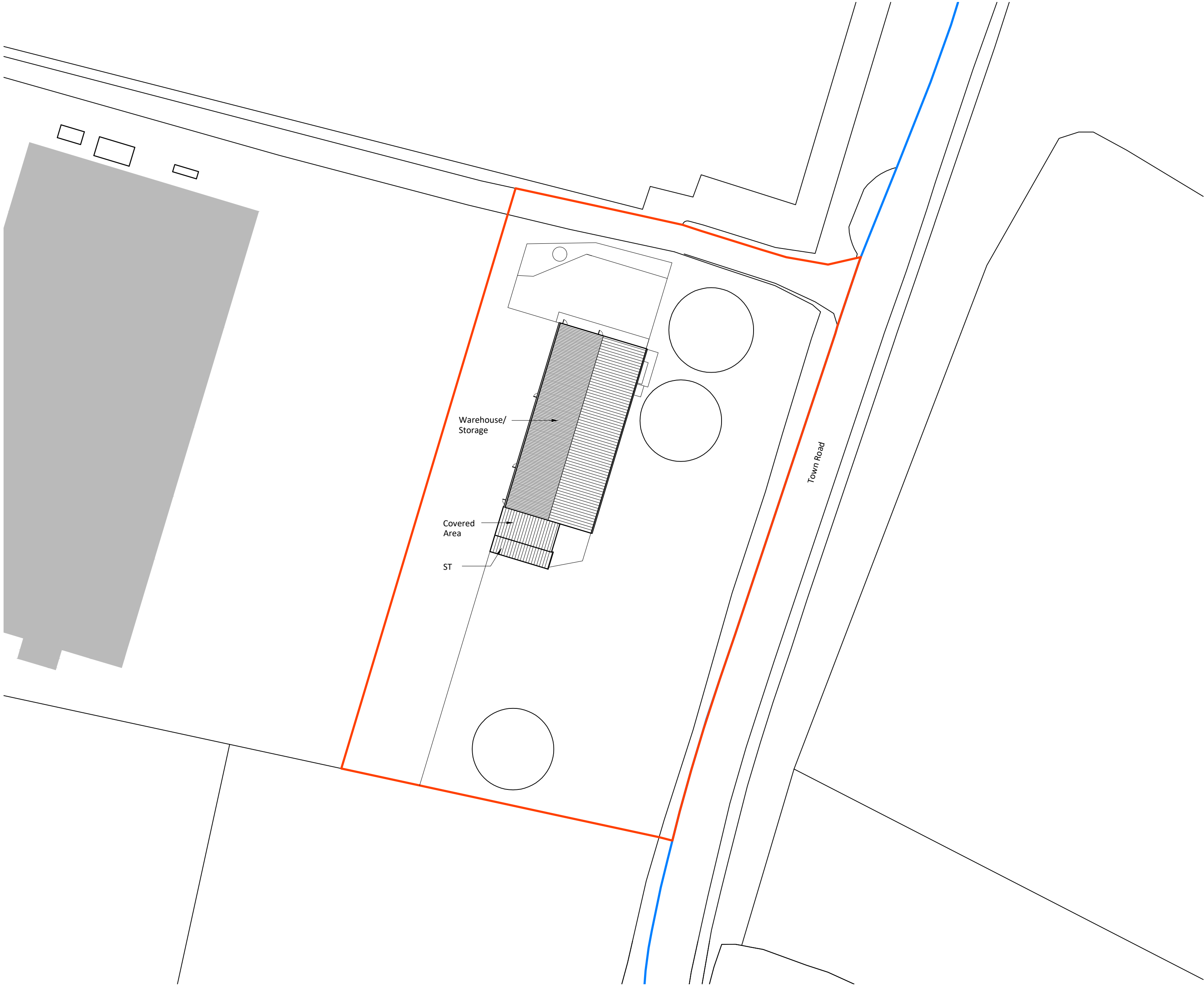
Existing Block Plan 1:500
