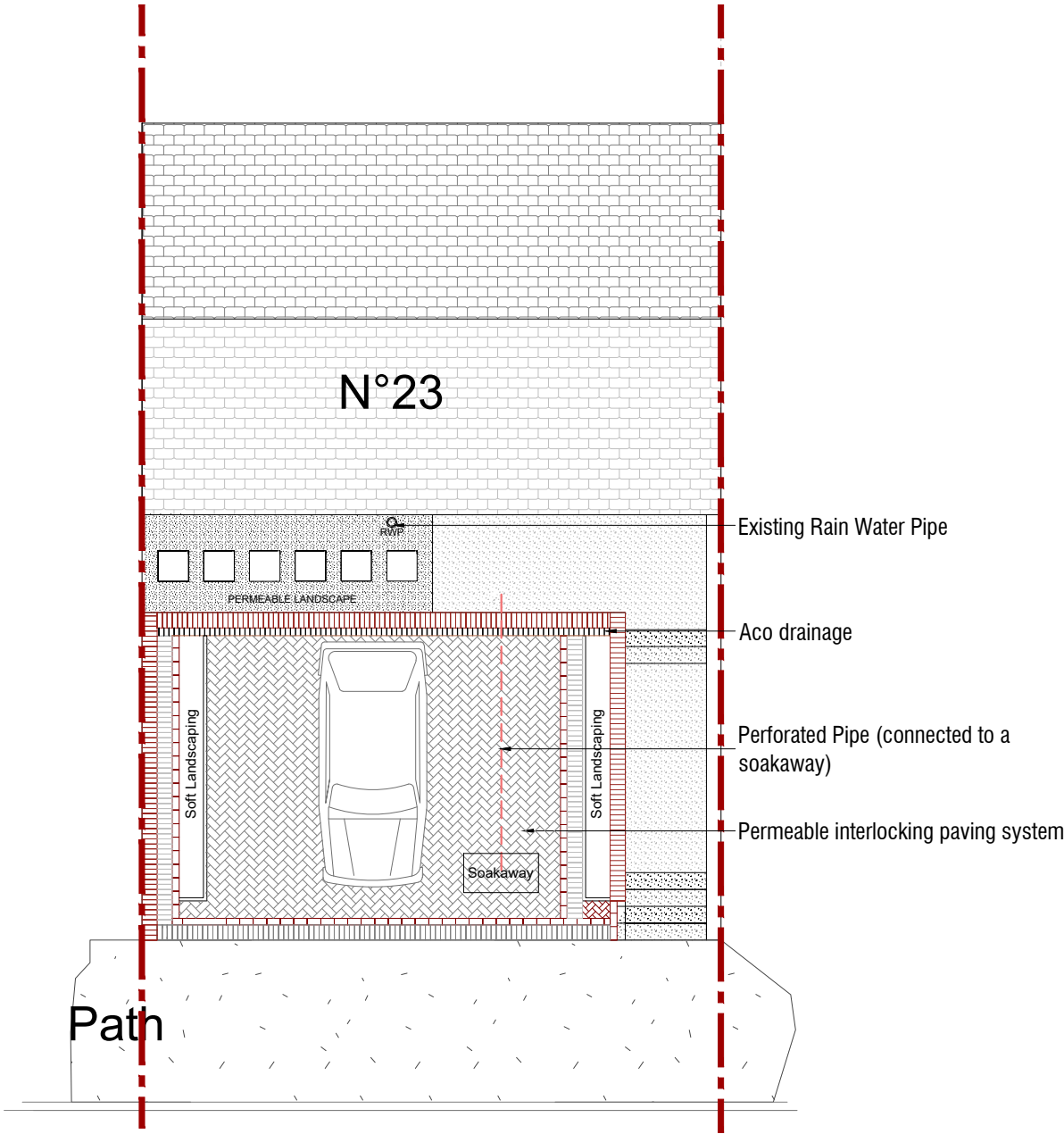
EXISTING FLOOR PLAN Scale 1:100
