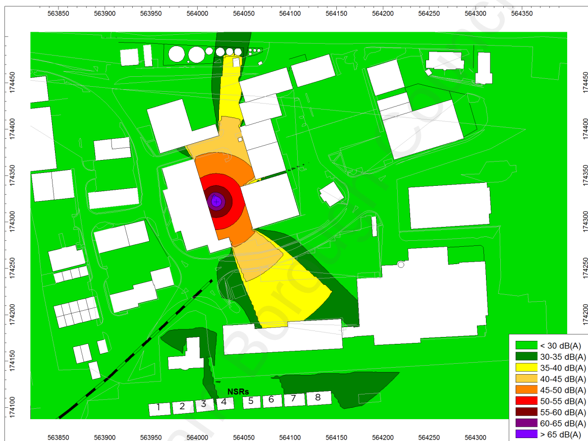
FIGURE 3: SPECIFIC SOUND LEVEL MAP
