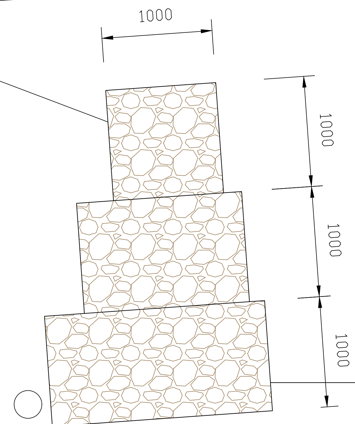
Section through new garden walls Caged gabion baskets
