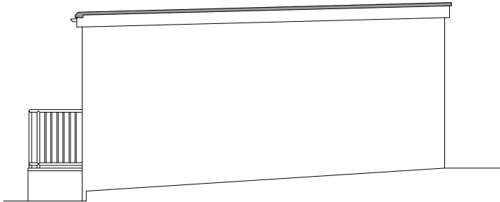
North Elevation (Side)
