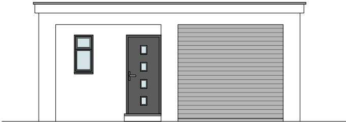
Front Elevation (West)
