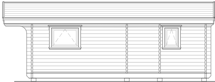
Rear Elevation
