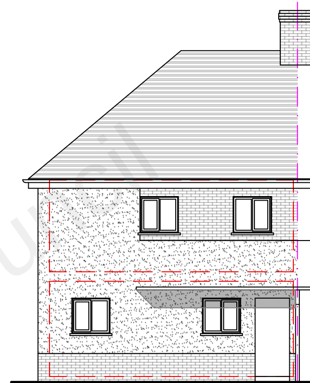
EXISTING FRONT (North East) ELEVATION
