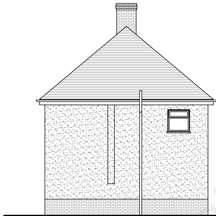
EXISTING SIDE (South East) ELEVATION
