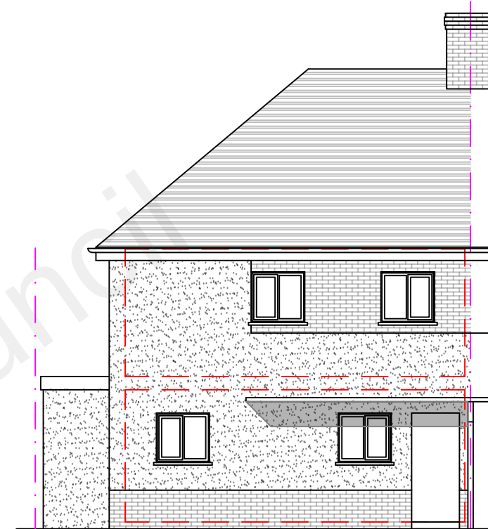
PROPOSED FRONT (North East) ELEVATION
