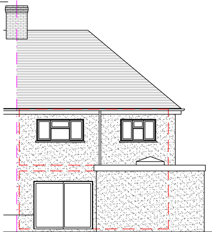
PROPOSED REAR (South West) ELEVATION
