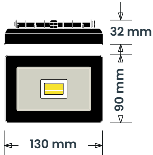
Floodlight Detail Scale 1:5
